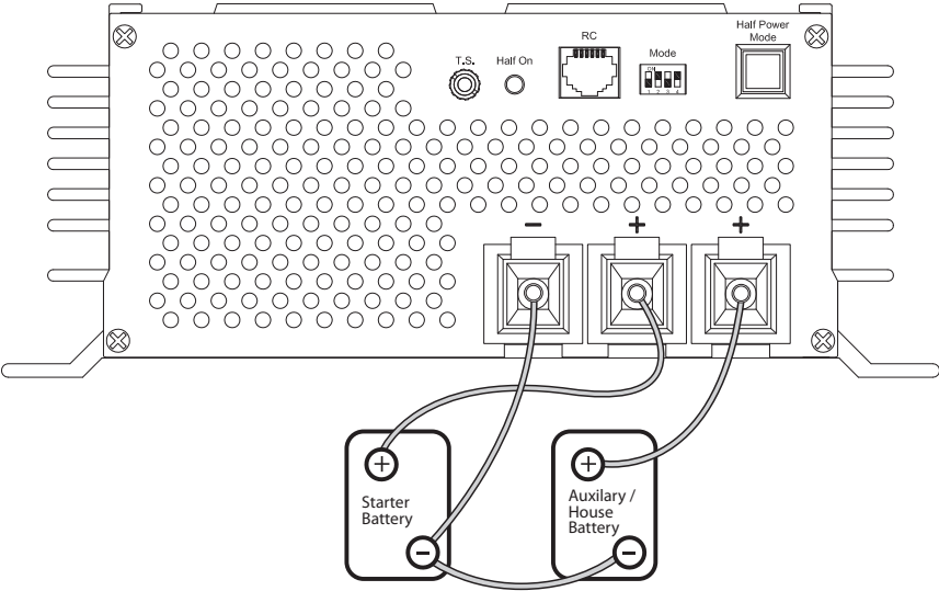
Fig. 7.1 Connecting 2 separate battery systems to 2 separate banks
