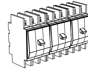
3 x 3-pole, 60 Amp 120/208 VAC circuit breakers (Square D QOU360)
