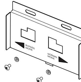
Three-phase bypass interlock plate and mounting hardware
